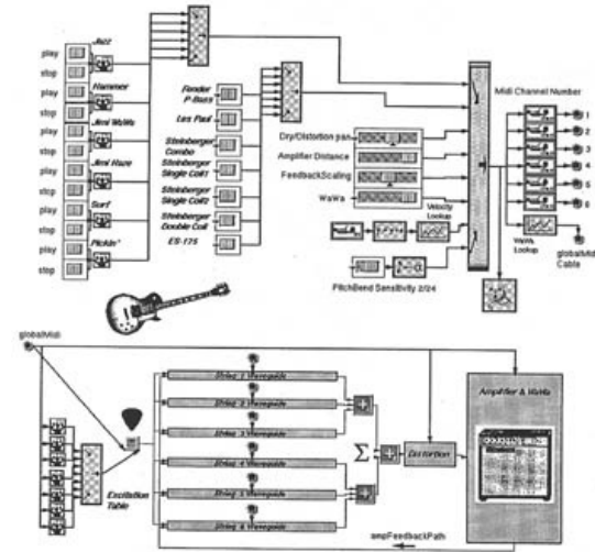
A six string electric guitar model with distortion, feedback and waha, implemented in SynthBuilder. This model runs on a single 72Mhz Motorola 56002 DSP.
